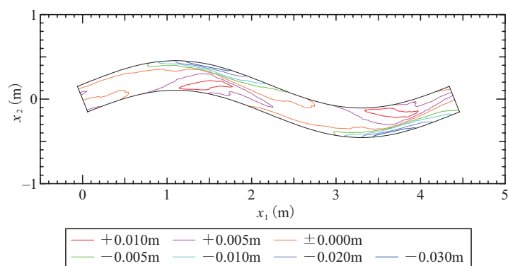
Fig. 27 河床形状の実験値 (西本ら, 1992) Experimental river bed forms
