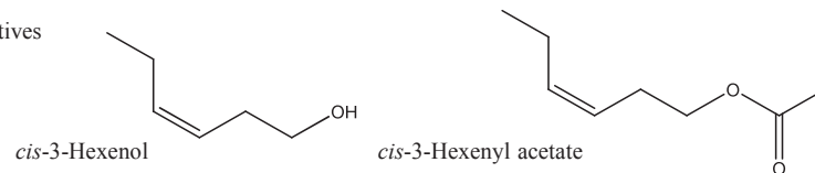
Fig. 2. Structures of major scent compounds of mints.
