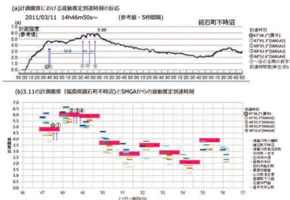
Fig.60 東北地方太平洋沖地震の計測震度と強震動域有為波の到達 (福島県鏡石町不時沼) Relationships between measurement seismic intensity (5 seconds type) and arriving time of affecting seismic waves from 4 each SMGA at Fujinuma, Kagamiishi, Fukushima Prefecture during the 2011 off the Pacific coast of Tohoku Earthquake
