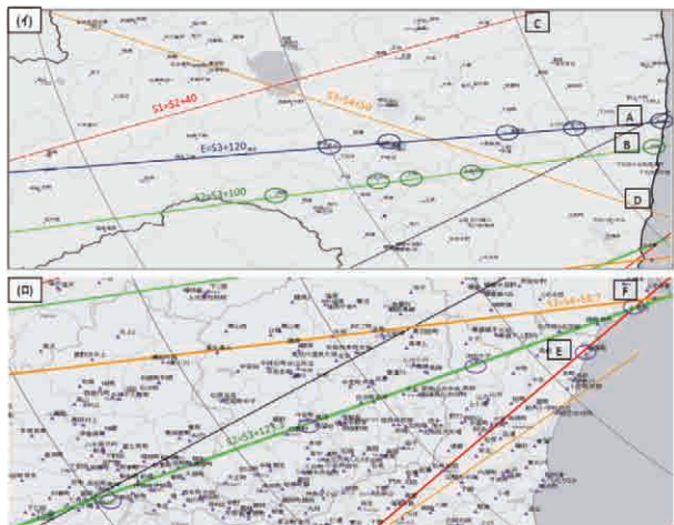
Fig.80 東北地方太平洋沖地震の観測点と震央・S3同時性(E=S3+120)ライン及び周辺ライン Location of survey stations and E=S3+120, S2=S3+100, S2=S3+123.3, & S3=S4+58.7 lines during 2011 off the Pacific coast of Tohoku Earthquake
