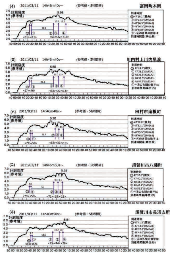
Fig.81 東北地方太平洋沖地震の震央・S3重合(E=S3+120)ライン上観測所の計測震度経過 Comparison of measurement seismic intensity (5 seconds type) and arrival time of affecting waves at survey stations on E=S3+120 line during 2011 off the Pacific coast of Tohoku Earthquake
