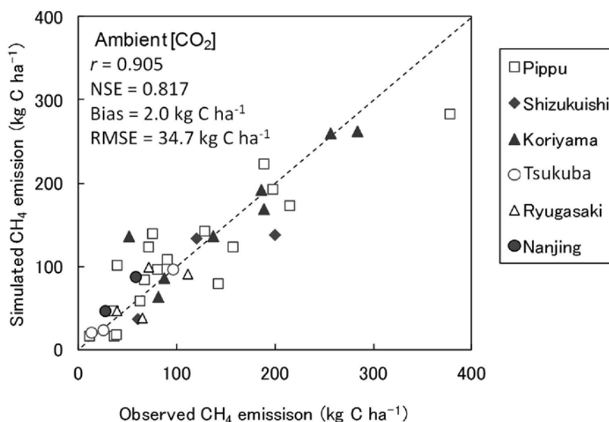
Fig. 7. Comparison between observed and simulated seasonal CH 4 emissions under ambient [CO 2 ] from the 6 sites of rice field.
