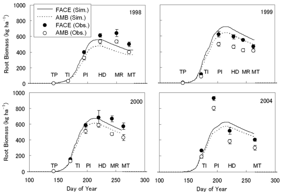
Fig. 20. Observed and simulated root biomass under elevated [CO_2] (FACE) and ambient [CO_2] (AMB). Values represent means \pm standard errors of the mean ( n = 4 ). Rice plant developmental stages on each sampling date are as follows: TP, transplanting; TI, tillering; PI, panicle initiation; HD, heading; MR, mid-ripening; MT, maturity. Observed data were compiled from Kim et al. (2001, 2003).
