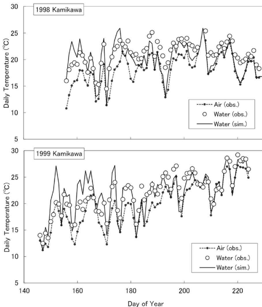
Fig. 6. Simulated paddy water temperature, along with observed air and paddy water temperatures at Pippu site in 1998 and 1999. Observed data of water temperature were compiled from Shimono (2003).
