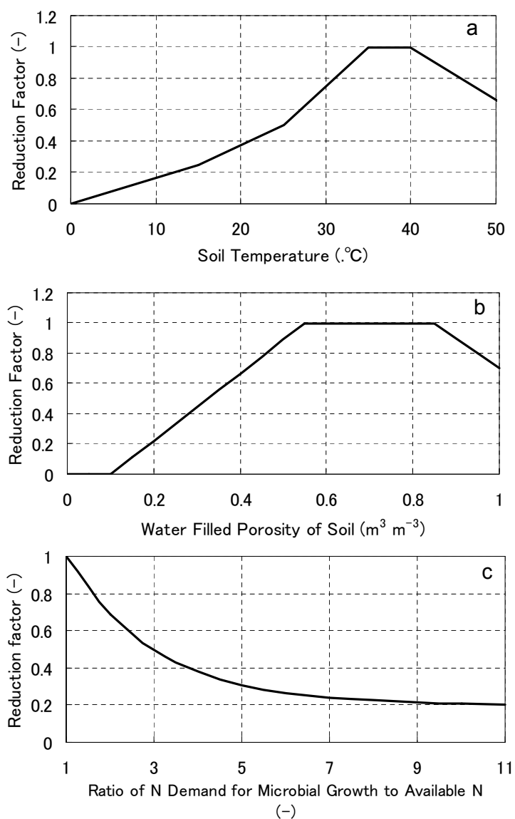
Fig. 4. Reduction factors for decomposition rate as a function of (a) soil temperature, (b) soil moisture, and (c) N deficiency.
