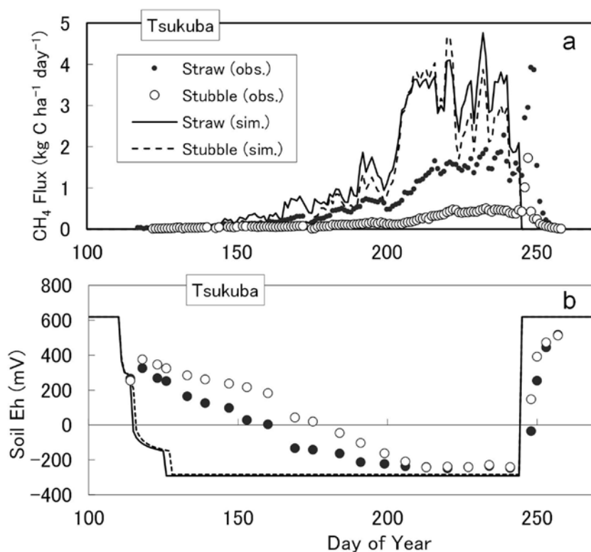
Fig. 23. Simulation of (a) daily methane flux and (b) soil Eh at the Tsukuba site by DNDC 8.2L.
