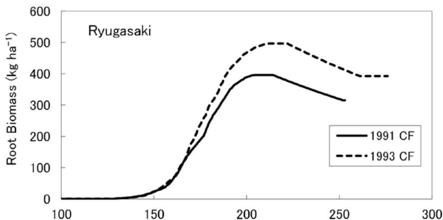
Fig. 17. Simulated root biomass under continuous flooding in 1991 and 1993 at the Ryūgasaki site.
