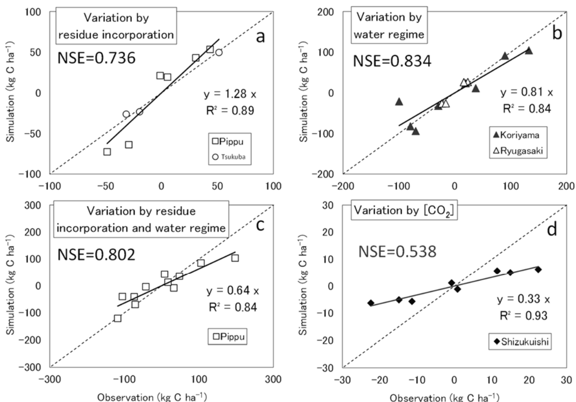
Fig. 8. Observed versus simulated variations in seasonal \text{CH}_4 emissions due to different treatments of (a) rice residue incorporation, (b) water management, (c) combination of residue incorporation and water management, and (d) atmospheric \text{CO}_2 concentration. Values of the x and y axes represent the difference from the mean of seasonal \text{CH}_4 emissions across all treatments at each site in each year (refer to equation 3.2 in the text).
