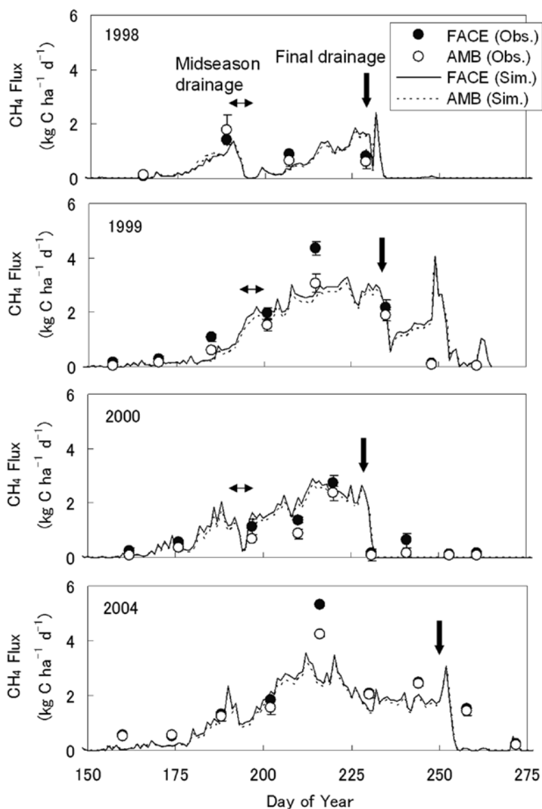
Fig. 22. Observed and simulated daily \text{CH}_4 fluxes under elevated [\text{CO}_2] (FACE) and ambient [\text{CO}_2] (AMB) at the Shizukuishi site. Values of observed flux represent means \pm standard errors of the mean ( n = 4 ). Horizontal and vertical arrows represent the midseason drainage and the date of the final drainage, respectively. Observed data for years 1998-2000 were compiled from Inubushi et al. (2003).
