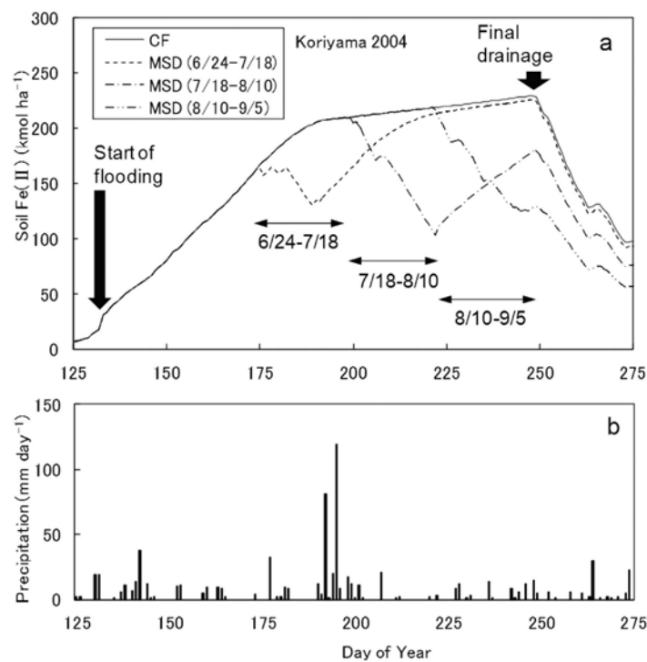
Fig. 16. (a) Simulated Fe(II) content in the 50 cm soil layer at the Koriyama site under different water managements in 2004 (CF, continuous flooding; MSD, midseason drainage). Horizontal bars ( ← → ) indicate the period of midseason drainage (dates represent month/day of the start and end of midseason drainage). (b) Observed daily precipitation at Koriyama in 2004.
