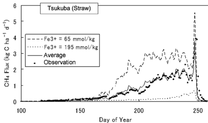
Fig. 11. Simulated daily \text{CH}_4 fluxes from the Straw plot at the Tsukuba site, assuming a hypothetical heterogeneous soil system. The soil was assumed to consist of regions with different concentrations of reducible Fe (65, 130 and 195 \text{mmol kg}^{-1} ), and the solid line represents the average of daily methane fluxes from those regions. Simulated methane flux assuming reducible Fe of 130 \text{mmol kg}^{-1} is shown in Fig. 3.4a.
