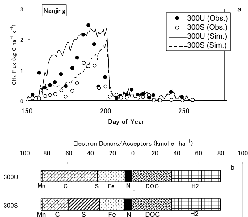
Fig. 10. (a) Observed and simulated daily \text{CH}_4 fluxes and (b) simulated electron budgets in 50 cm flooded soil layer at the Nanjing site. Observed data were compiled from Cai et al. (1997).
