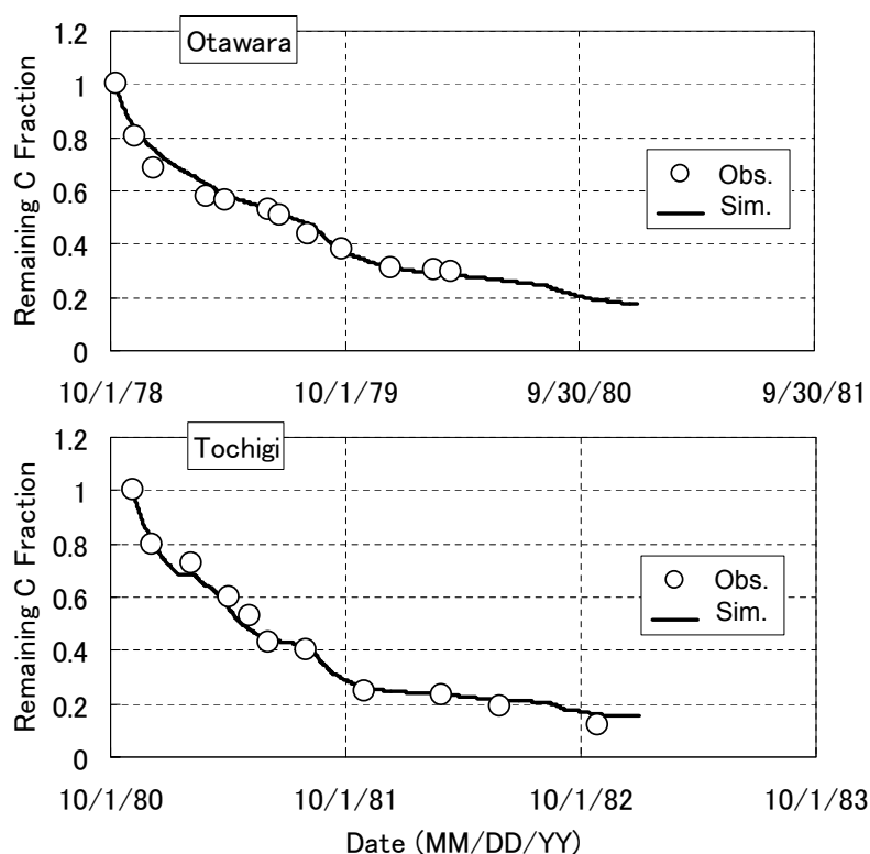
Fig. 5. Observed and simulated straw decomposition rates at two paddy fields in Tochigi prefecture, Japan. Observed data of straw decomposition were compiled from Mogi et al. (1980) and Yoshizawa and Nakayama (1983).
