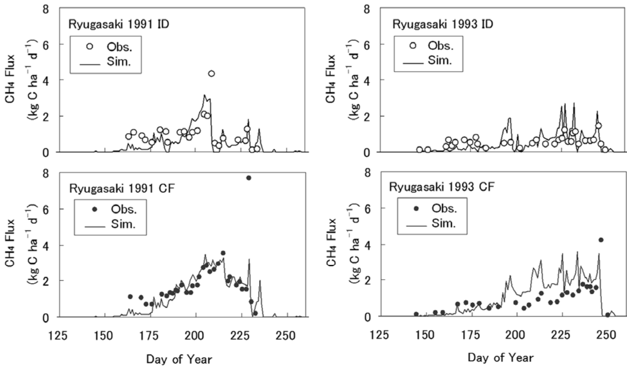
Fig. 13. Observed and simulated daily \text{CH}_4 fluxes from the Ryugasaki site under different water managements in 1991 and 1993 (CF, continuous flooding; ID, intermittent drainage). Observed data were compiled from Yagi et al. (1996).
