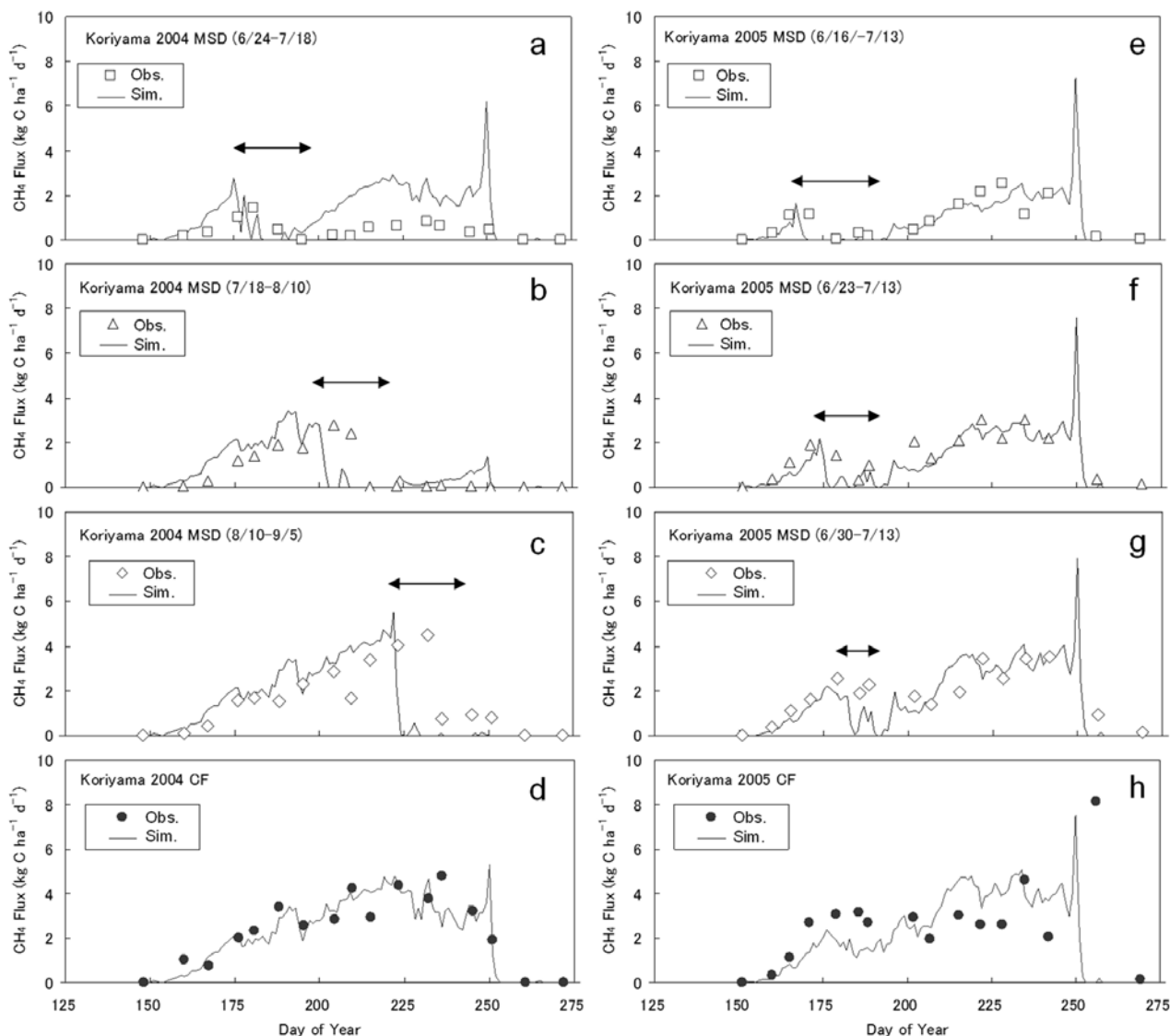
Fig. 12. Observed and simulated daily \text{CH}_4 fluxes from the Koriyama site under different durations or timings of midseason drainage in 2004 (a-d) and 2005 (e-h). CF and MSD stand for continuous flooding and midseason drainage, respectively. The dates in parentheses represent the month/day of the start and end of midseason drainage, and horizontal bars ( \longleftrightarrow ) indicate the periods of midseason drainage. Observed data were compiled from Saito et al. (2006).
