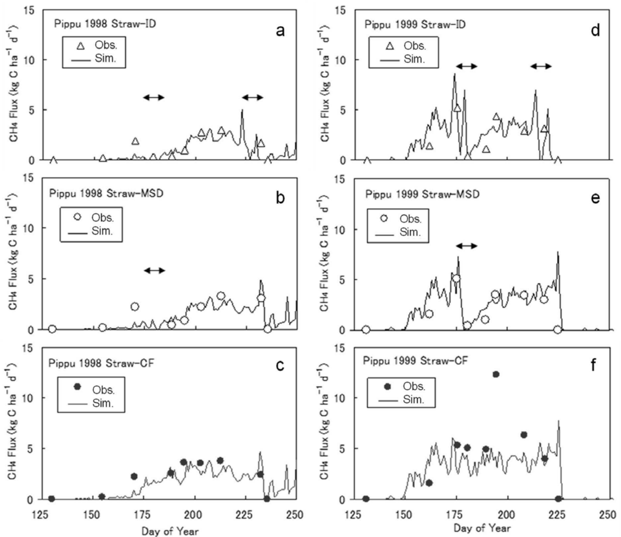
Fig. 18. Observed and simulated daily \text{CH}_4 fluxes from the Pippu site under different water managements with rice straw incorporation in years 1998 (a-c) and 1999 (d-f). CF, MSD and ID stand for continuous flooding, midseason drainage and intermittent drainage, respectively. Horizontal bars ( \leftrightarrow ) indicate the periods of midseason drainage or intermittent drainage. Observed data were compiled from Goto et al. (2004).
