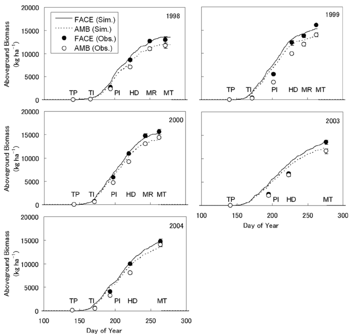
Fig. 19. Observed and simulated aboveground biomass under elevated [\text{CO}_2] (FACE) and ambient [\text{CO}_2] (AMB). Values represent means \pm standard errors of the mean ( n = 4 ). Rice plant developmental stages on each sampling date are as follows: TP, transplanting; TI, tillering; PI, panicle initiation; HD, heading; MR, mid-ripening; MT, maturity. Observed data were compiled from Kim et al. (2001, 2003).
