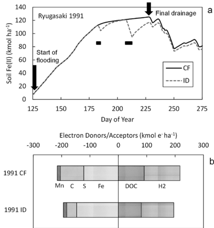
Fig. 15. (a) Simulated soil Fe (II) content and (b) simulated electron budgets in 50 cm flooded soil layer at the Ryugasaki site under different water managements in 1991 (CF, continuous flooding; ID, intermittent drainage). Horizontal bars in the upper graph indicate the periods of intermittent drainage.
