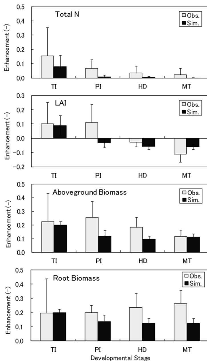
Fig. 21. Observed and simulated relative enhancement of rice plant variables under FACE compared to ambient [CO_2] at different developmental stages (TI, tillering; PI, panicle initiation; HD, heading; MT, maturity). Values indicate the average and standard deviation over all years at the Shizukuishi site.
