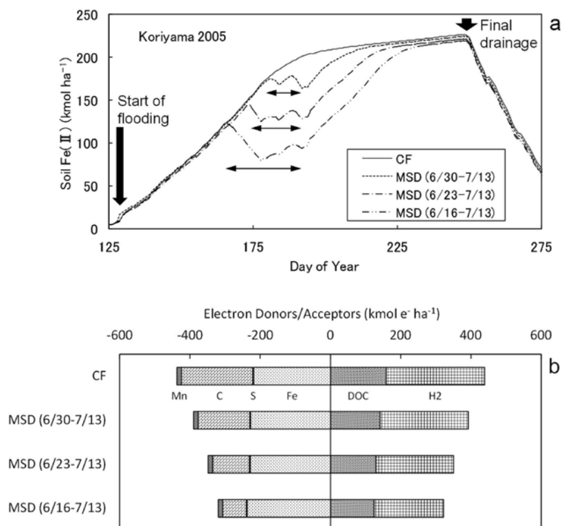
Fig. 14. (a) Simulated soil Fe (II) content and (b) simulated electron budgets in 50 cm flooded soil layer at the Koriyama site under different water managements in 2005 (CF, continuous flooding; MSD, midseason drainage). Horizontal bars ( ← → ) indicate the period of midseason drainage for each water management (dates represent month/day of the start and end of midseason drainage).
