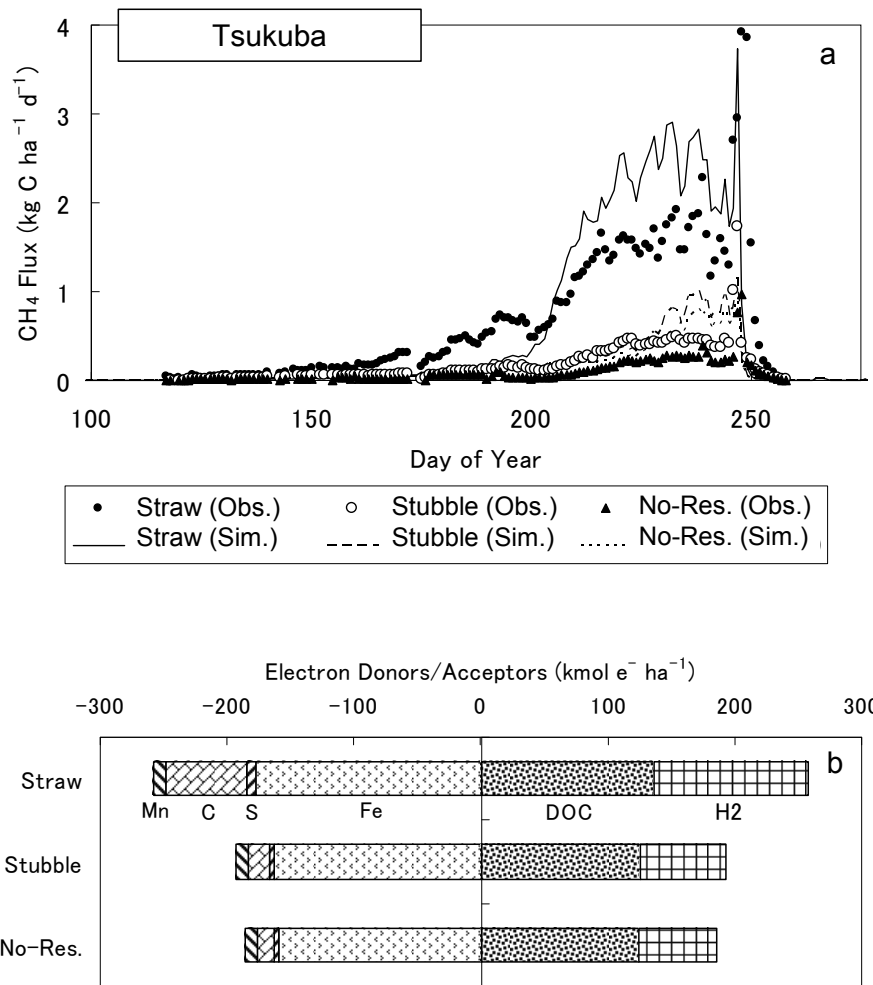
Fig. 9. (a) Observed and simulated daily CH 4 fluxes, and (b) simulated seasonal electron budgets in 50 cm flooded soil layer for different rice residue incorporation at the Tsukuba site.
