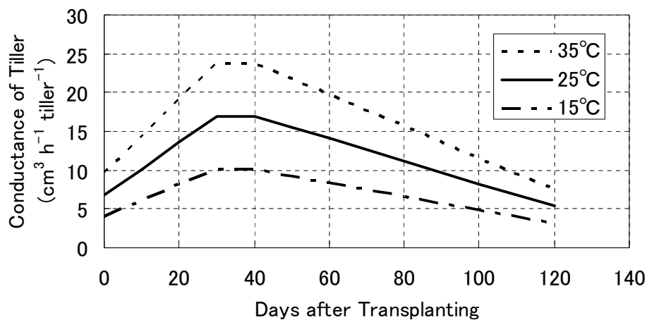
Fig. 3. The function to estimate the conductance of rice tillers for CH 4 as a function of plant age and soil temperature.
