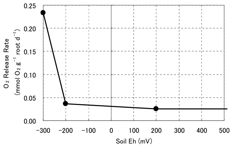
Fig. 2. The function to calculate the oxygen release rate from rice roots as a function of soil redox potential (Eh).
