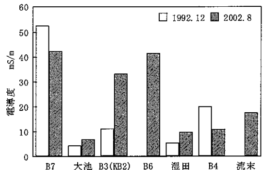
Fig.11 電導度の比較 Electrical Conductivity
