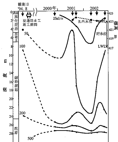
Fig.9 B6 の電導度変化 Electrical Conductivity in B6
