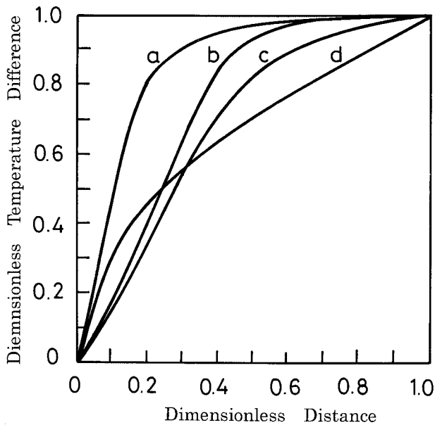
Fig. 4 Dependence of temperature changes ( T/T_{\max} ) dimensionless by maximum temperature change ( T_{\max} ) on dimensionless fetch ( x/X ) under 4 conditions. T_{\max} denotes the temperature changes ( T_{\max} ) at maximum fetch ( X ) of experimental field.
