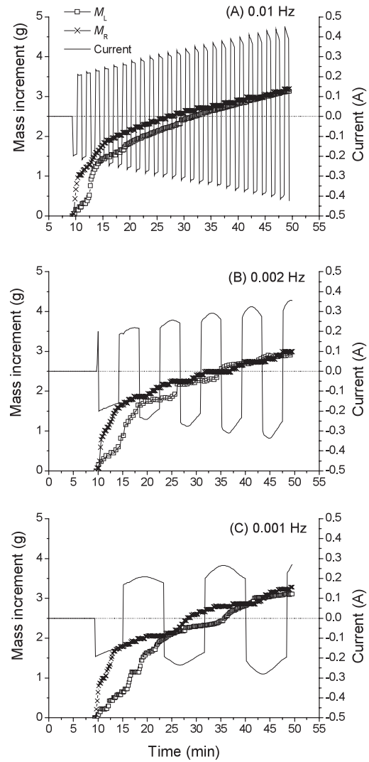
Fig. 9. Drainage mass increment as well as current change with time and frequencies
