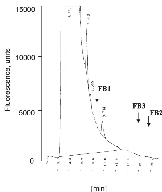
Fig 1. b) HPLC-FL chromatogram of rice seed extract # 1
