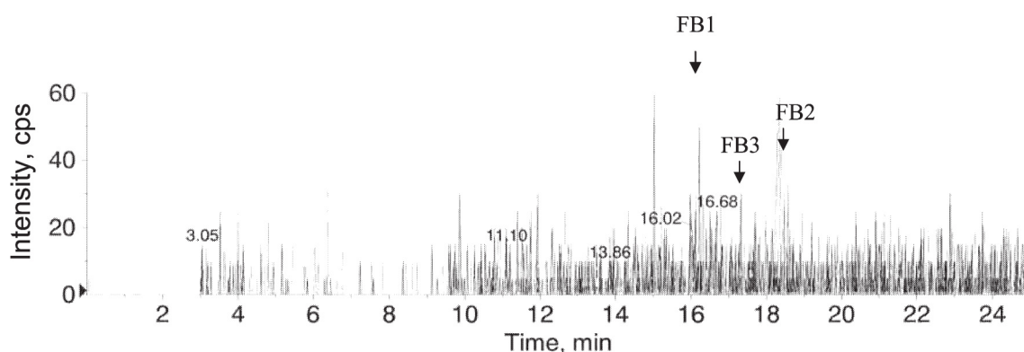
Fig 2. b) LC-MS/MS chromatogram of rice seed extract # 2
