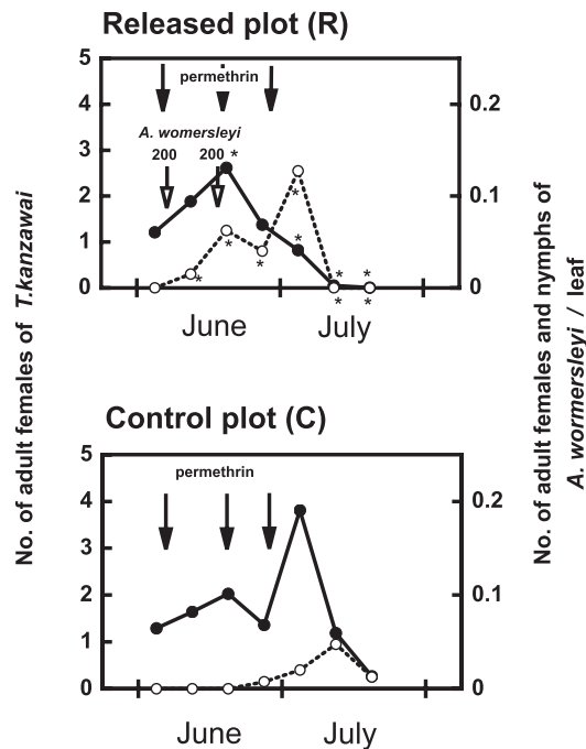
Fig. 12 Effect of the release of the predatory mite A. womersleyi (-----) resistant to synthetic pyrethroid on the suppression of the Kanzawa spider mite T. kanzawai (—) in a netted house (5×5m). Two hundreds of adult females were inoculated in each release. Asterisks on the graph in the released plot indicate a significant difference in the density of each species between the two plots ( p < 0.05 , Wilcoxon two sample test).
