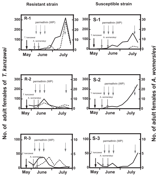
Fig. 11 Comparison of population changes in the Kanzawa spider mite T. kanzawai (—) and the two strains (resistant and susceptible) of the predatory mite A. womersleyi (-----) under synthetic pyrethroid application to tea planted in a pot (30 cm in diameter).
