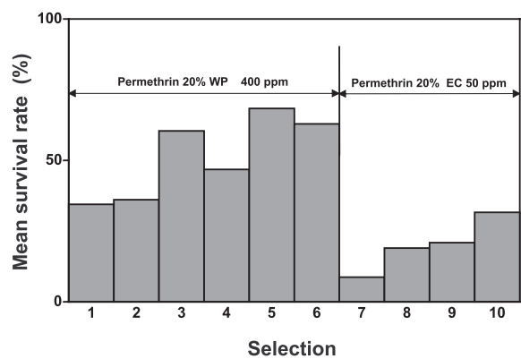
Fig. 7 Response of adult female A. womersleyi (Hiranuma-1 strain) to selection with permethrin. Permethrin (WP) of 400 ppm was used during the selections 1-6, and permethrin (EC) of 50 ppm during the continuing selections 7-10. The 500-900 adult females were divided into 2-4 groups and treated with permethrin in each selection.
