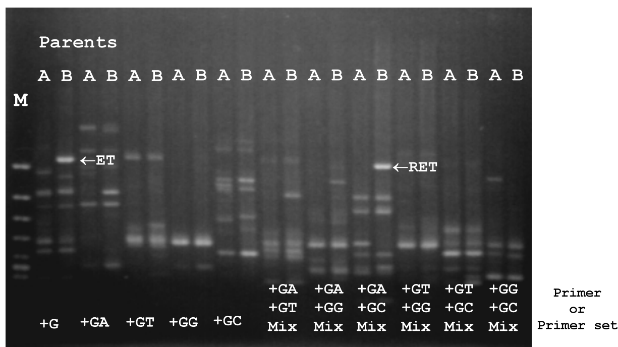
Fig. 7 Electropherogram of PCR products used for repeat search for e-RAPD.
