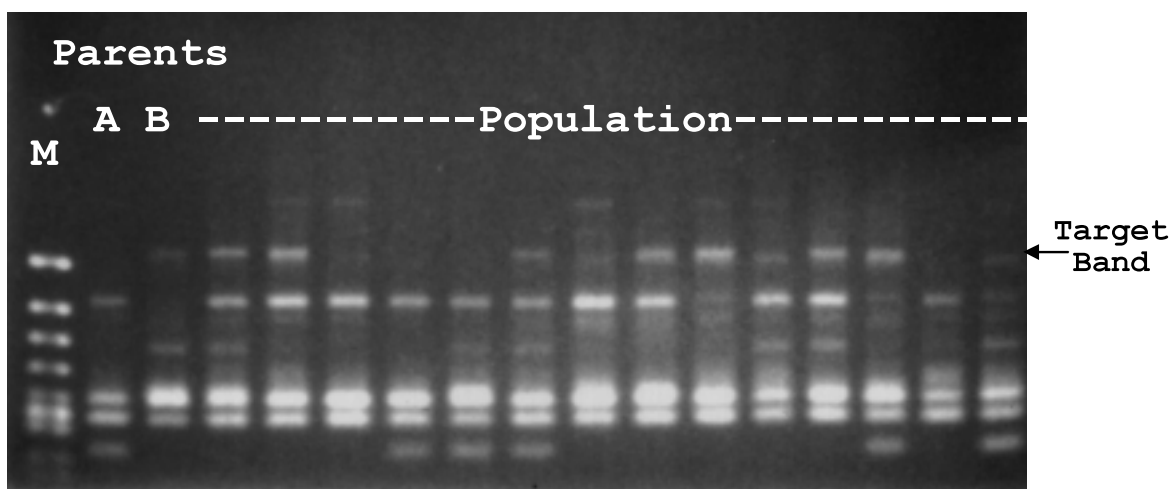
Fig. 3 Original RAPD patterns in the F_1 segregating population of tea. M: DNA size marker ( \phi X174/ Hinc II digest).
