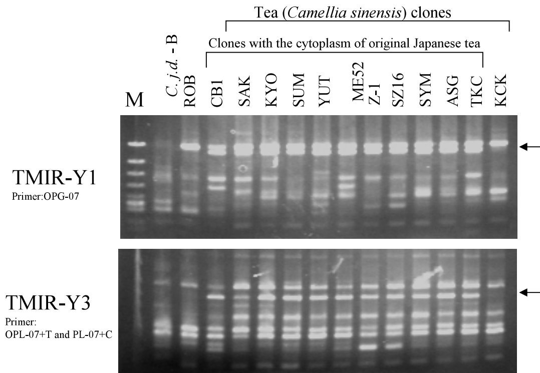
Fig. 17 Maternally inherited RAPD (TMIR - Y1) and e - RAPD (TMIR - Y3) band patterns of C. japonica var. decumbens , 'Robiraki' and C. sinensis (tea) clones that have the cytoplasm of original Japanese tea. M: DNA size marker ( \phi X174/ HincII digest), C. j. d. -B : C. japonica var. decumbens clone 'Yukitsubaki - B', ROB: 'Robiraki', CB1: 'Chatsubaki No.1' ( C. sinensis \times C. japonica ), SAK: 'Sayamakaori', KYO: 'Kyomidori', SUM: 'Samidori', YUT: 'Yutakamidori' ME52: 'ME52', Z-1: 'Z-1', SZ16: 'Shizu - zai16', SYM: 'Sayamamidori', ASG: 'Asagiri', TKC: 'Takachiho', KCK: 'Kana - Ck17'.
