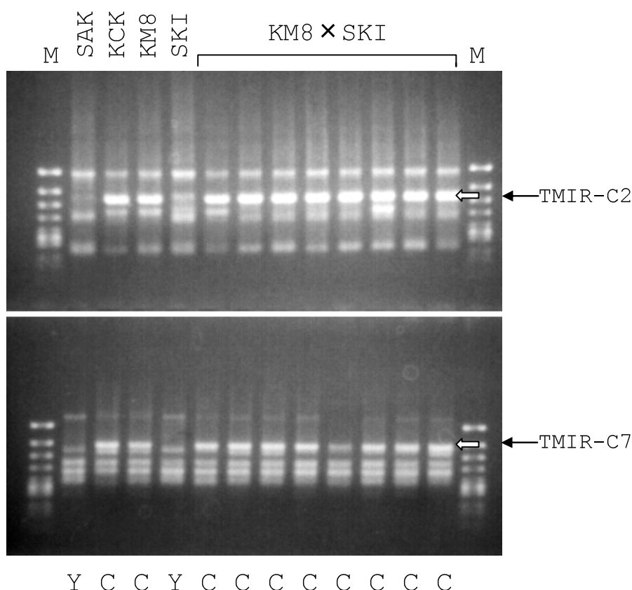
Fig. 10 Genetic inheritances of the maternally inheritable RAPD derived from tea clonal strain 'Kana-Ck17'. M: DNA size marker ( \phi X174/ HincII digest), SAK: 'Sayamakaori', KCK: 'Kana-Ck17', KM8: 'KM8', SKI: 'Sakimidori'. Symbols of Y and C at the bottom of the photograph indicate the clones considered to be same cytoplasm to 'Yabukita' and 'Kana-Ck17' from their pedigree records, respectively.
