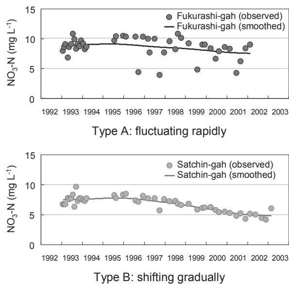
Fig. 15 Categorization of fluctuations of \text{NO}_3\text{-N} concentrations
