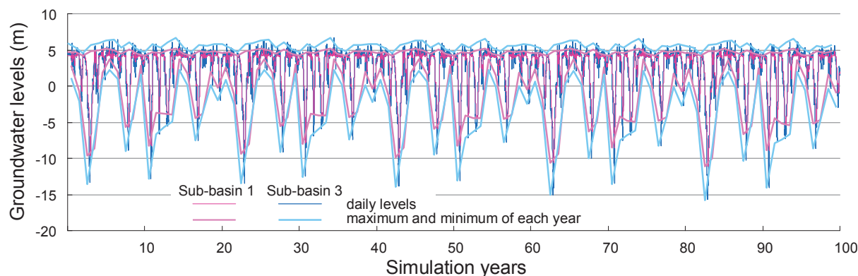
Fig. 36 Simulated groundwater levels for the 100 years
