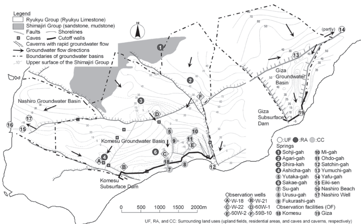
Fig. 19 Geological settings and the sampling sites (Okinawa General Bureau, 2006)
