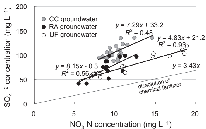
Fig. 24 Relationship between the concentrations of \text{NO}_3\text{-N} and \text{SO}_4^{2-} in the study area
