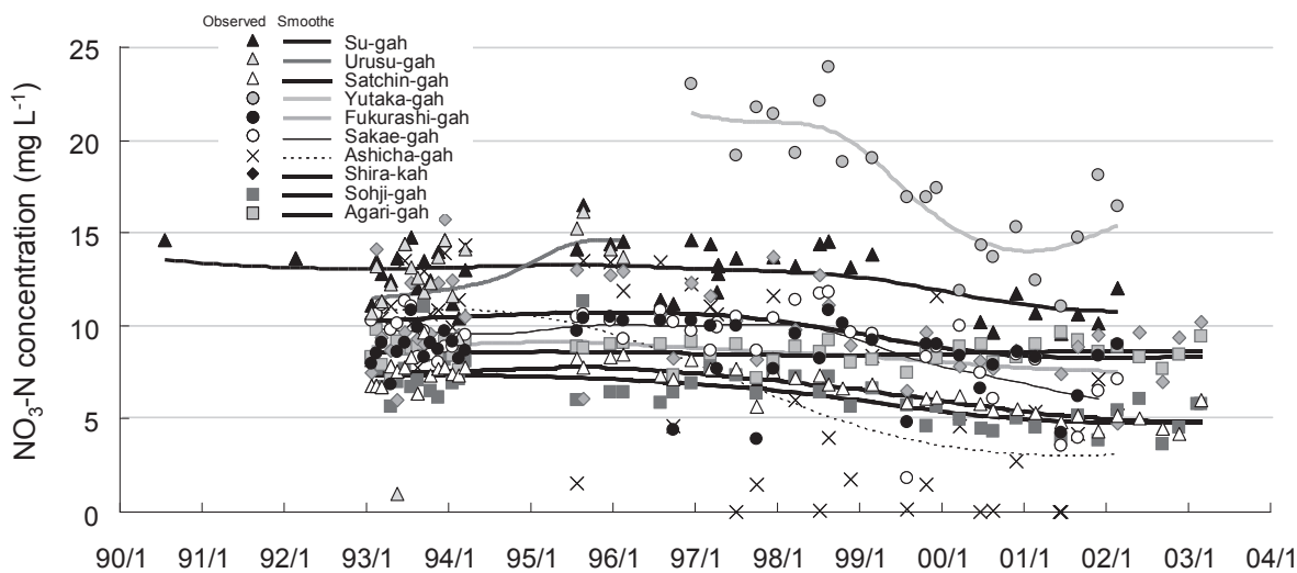
Fig. 14 Observed \text{NO}_3\text{-N} concentrations in spring waters
