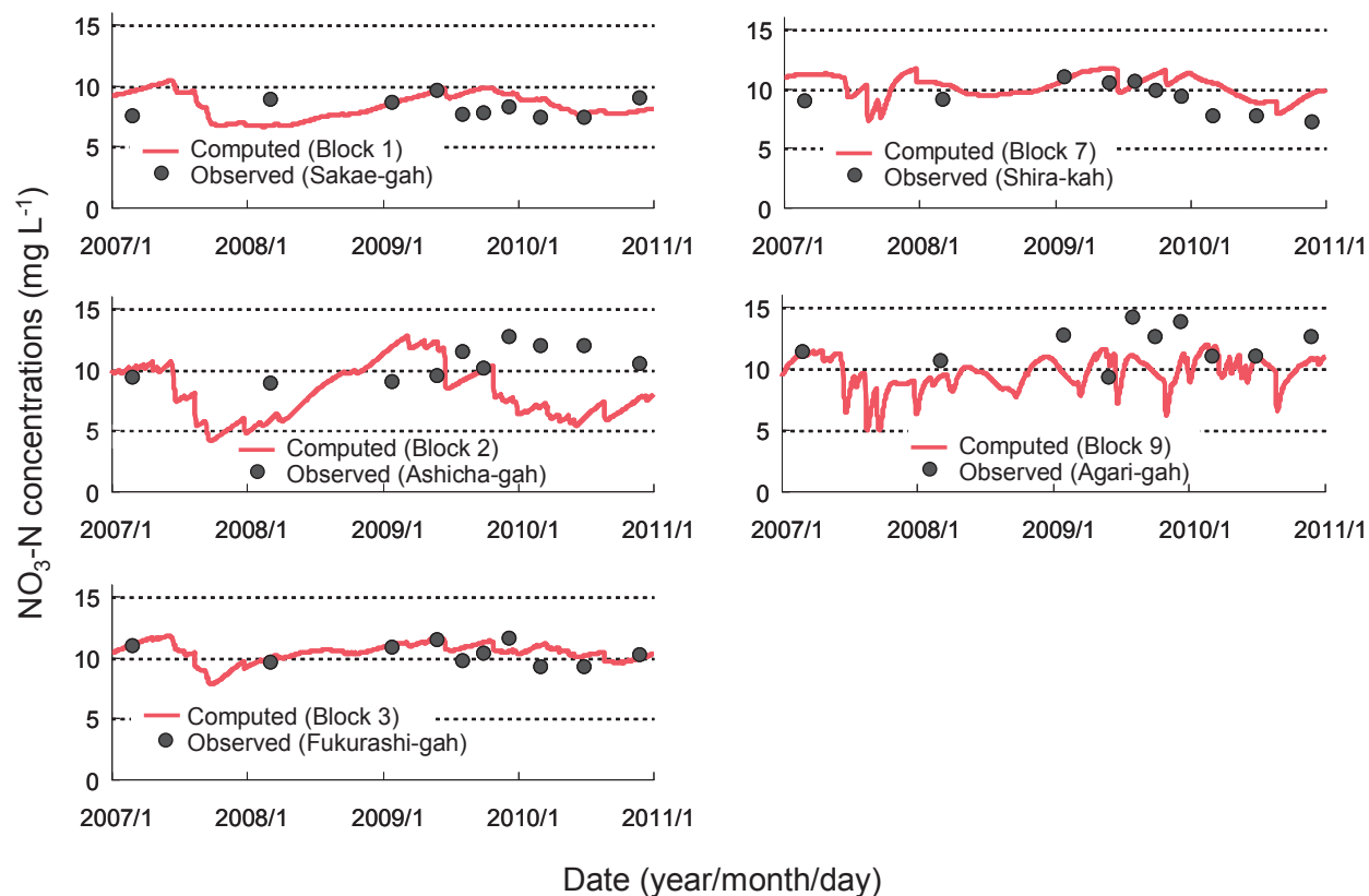
Fig. 34 Observed and computed \text{NO}_3\text{-N} concentrations in groundwater after the dam construction
