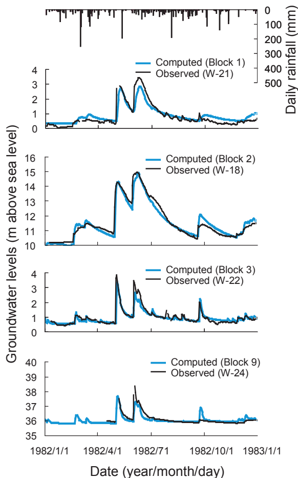
Fig. 31 Observed rainfall and observed and computed groundwater levels before the dam construction
