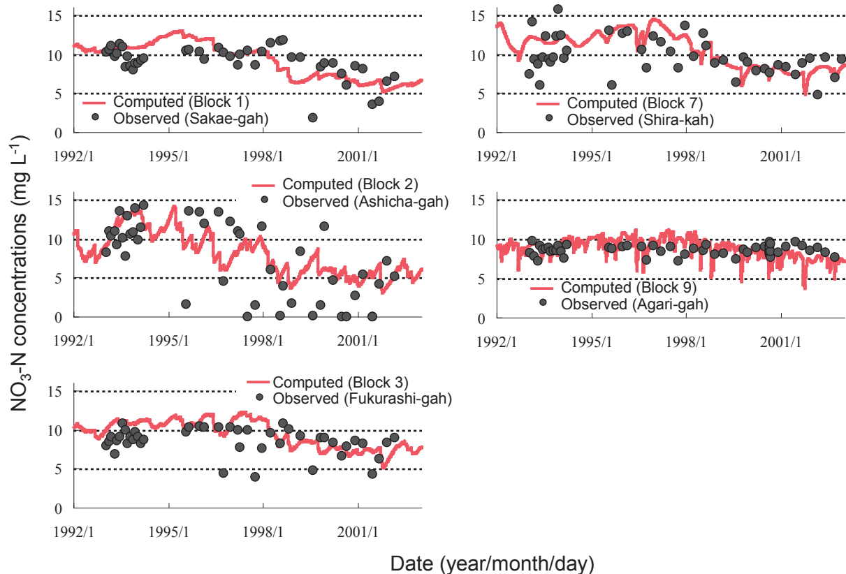
Fig. 33 Observed and computed \text{NO}_3\text{-N} concentrations in groundwater before the dam construction
