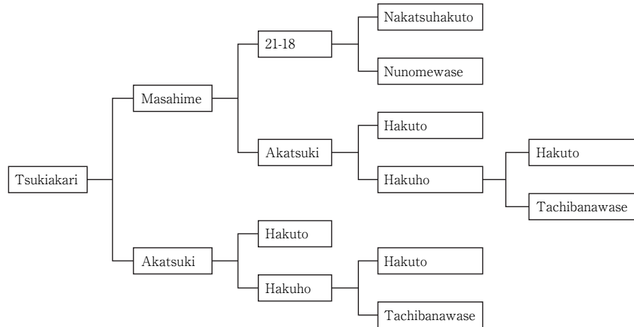
Fig. 1 Pedigree of 'Tsukiakari' peach
