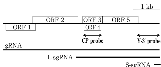
Fig. 2 Genome organization of SbDV
