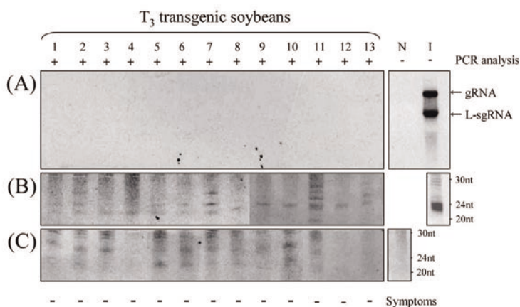
Fig.10 Detection of SbDV virion in T 3 soybean plants by northern blot hybridization analysis with the CP probe and accumulation of SbDV-CP homologous siRNA before and after inoculation with SbDV.
