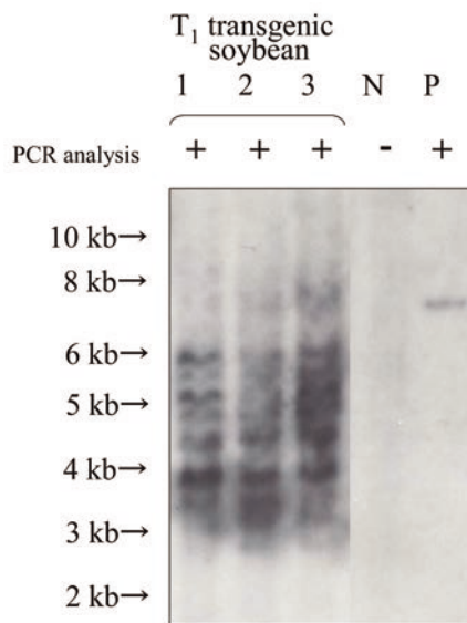
Fig. 7 Southern blot hybridization analysis of T 1 soybean plants. Genomic DNA (5 µg) was digested with Eco RI, separated in 0.8% agarose gel, blotted onto membrane, and hybridized with CP gene probe. 'N', non-transformed soybean (cv. Jack); 'P', positive control (pCP/IR/G digested with Eco RI). 'PCR analysis' shows the presence or absence of amplified, 592-bp, SbDV- CP transgene PCR product.
